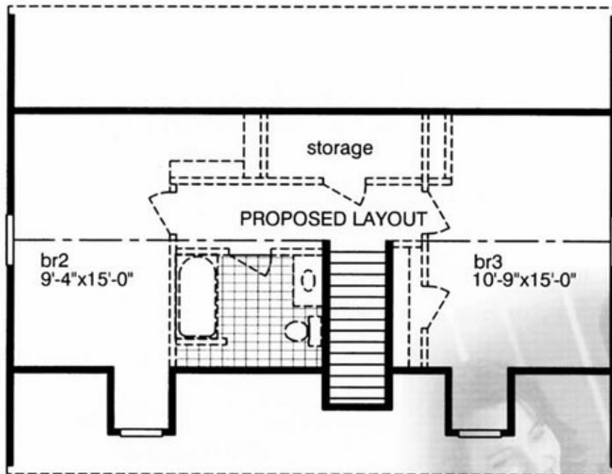
2nd Level
